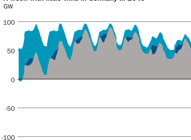
A week with little wind in Germany in 2040
