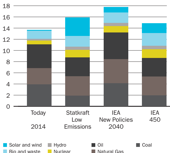
Global primary energy demand (Billions toe)
