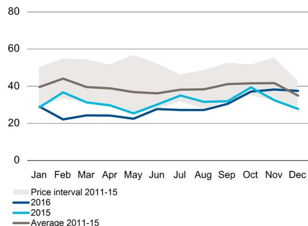
EEX Germany, spot price (base) EUR/MWh
